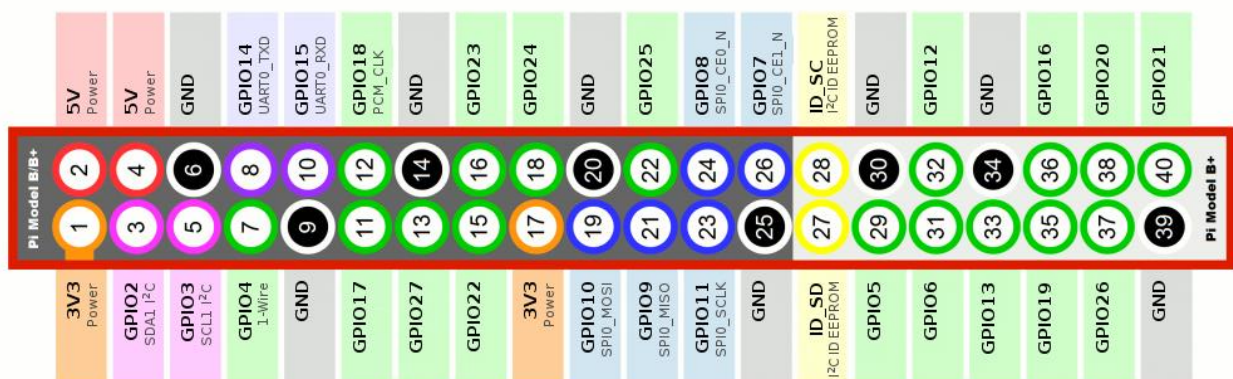
Figura 11 Pinos GPIO Raspberry Pi
